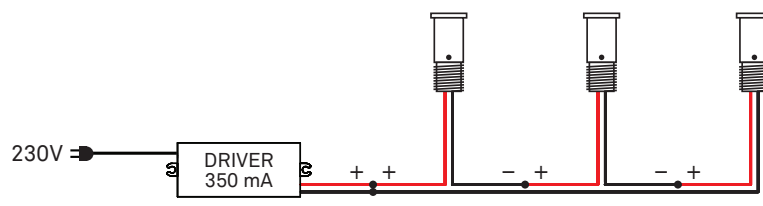
Connection scheme with several fixtures (series connection):
